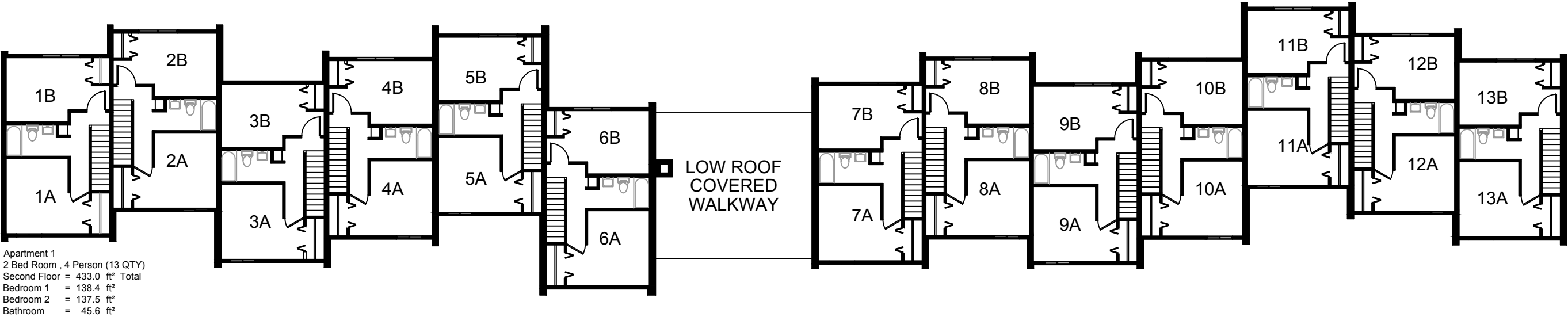
SECOND FLOOR
